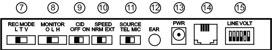
REAR PANEL
